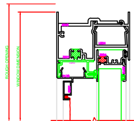
104 HEAD SERIES: 3500
