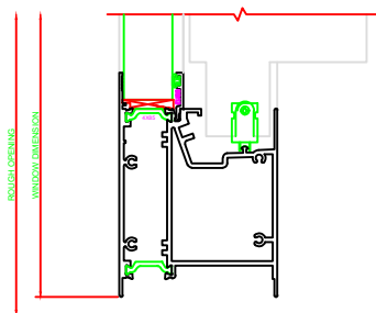
201 SILL SERIES: 3500
